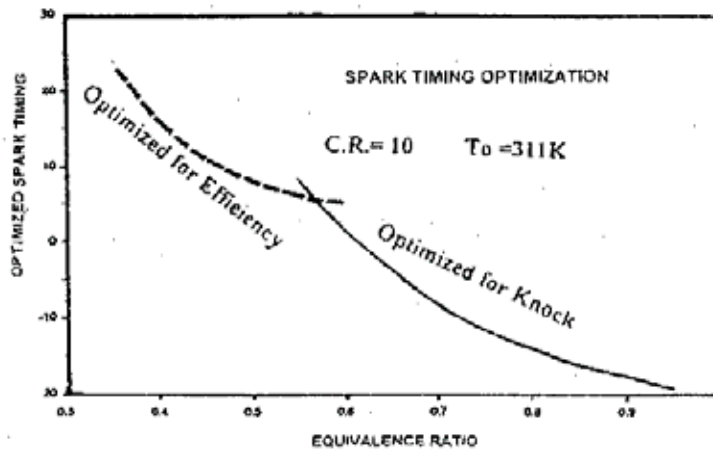
Fig. 4. Typical variations in spark timing for optimum efficiency and avoidance of knock for lean mixture operation with hydrogen, [14]
