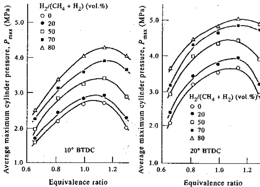
Fig. 6. Typical variations in the maximum cylinder pressure with changes in equivalence ratio when operating on a range of fuel mixtures of hydrogen and methane for two spark timings, [18]
