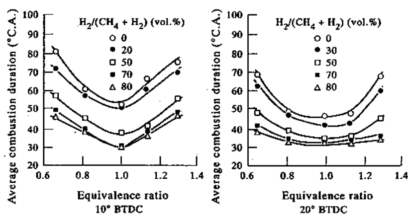
Fig. 1. Typical variations in the length of the combustion period in degrees with equivalence ratio for a range of H 2 -CH 4 mixtures for two spark timings at a compression ratio of 8.5:1 and 900 rev/min, [18]
