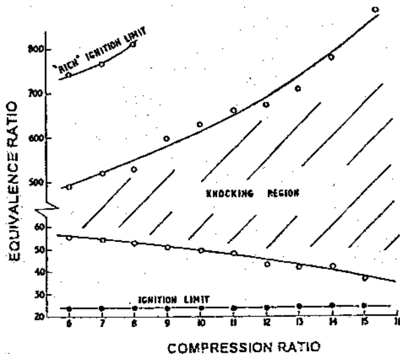
Fig. 7. Variations of operational limits for ignition and knock with compression ratio changes for hydrogen operation at ambient intake conditions, [20]
