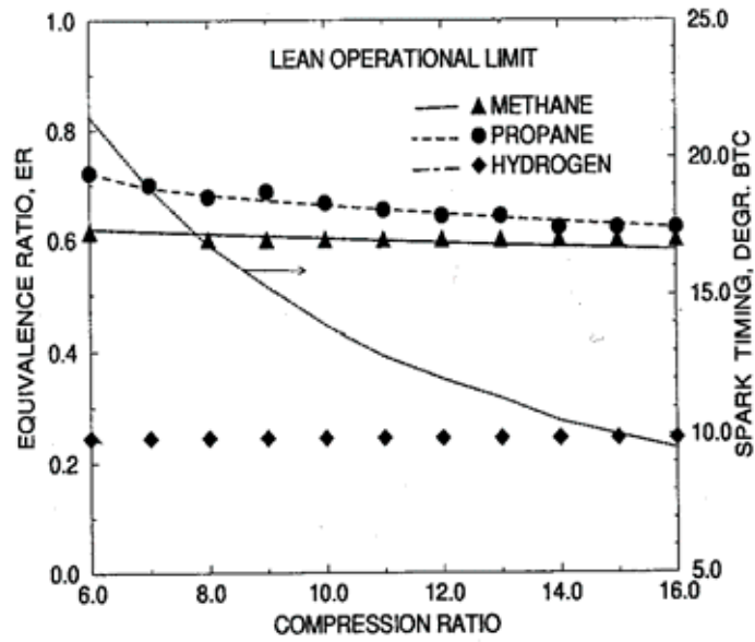
Fig. 2. Variations of the lean operational limits with changes in compression ratio for different gaseous fuels at 900 rev/min, [13]
