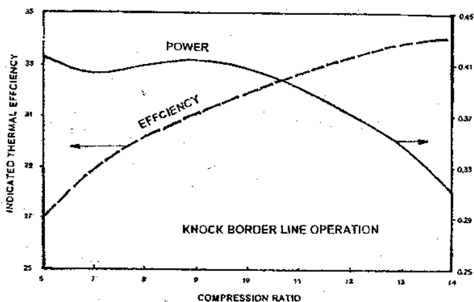
Fig. 5. Typical variations in indicated power output and efficiency with changes in compression ratio when using optimum spark timing for borderline knock, [14]
