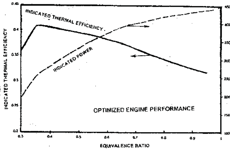
Fig. 3. Typical variations in the indicated power output and efficiency with leaning of equivalence ratio for hydrogen operation using optimum spark timing, [14]
