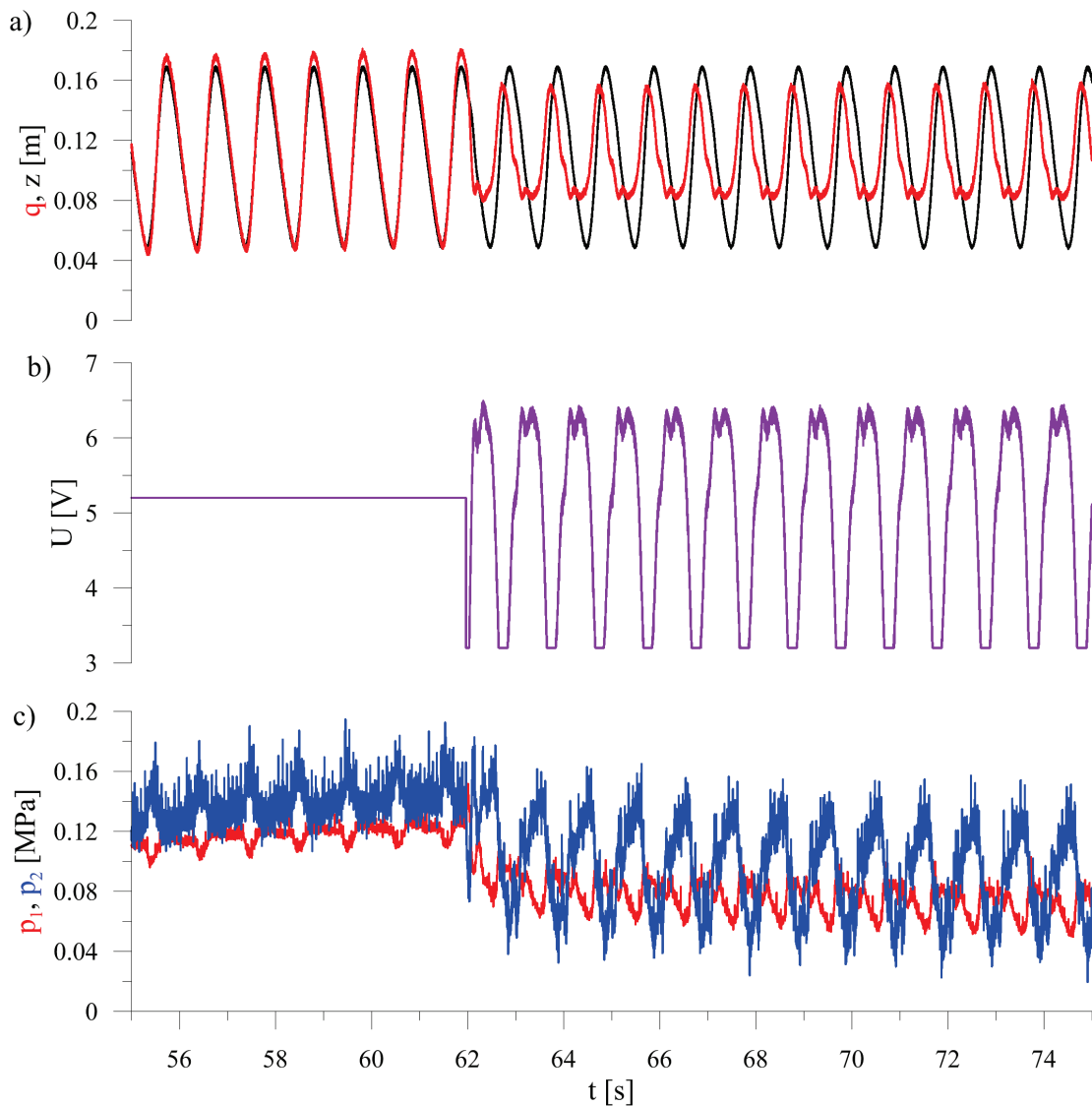
Fig. 7. Waveforms of: a) the vertical vibrations operator's seat versus base vibrations, b) controlling the mass flow rate of air supplying the actuator using the voltage signal from a servo-valve, c) pressure p_1, p_2 in cylinder chambers
