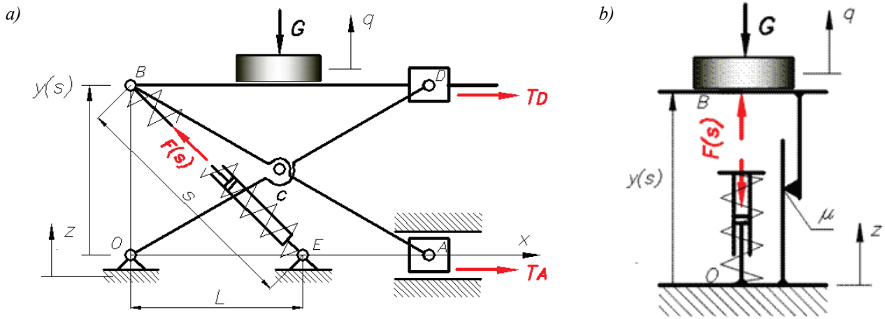
Fig. 1. Kinematic system of the seat suspension (a). Replacement model of the active seat suspension (b)
