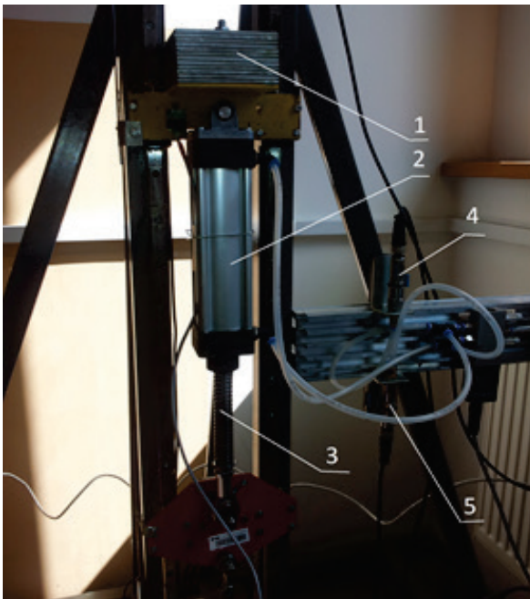
Fig. 4. General view of the test stand: 1 – weight G , 2 – pneumatic cylinder, 3 – spring, 4, 5 – pressure transducer
