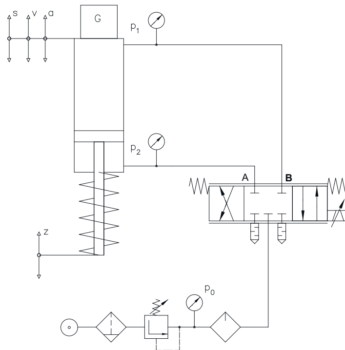
Fig. 3. Schematic diagram of control of the pneumatic cylinder
