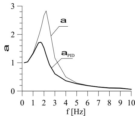
Fig. 2. Transmissibility function of a regulated single-acting pneumatic actuator
