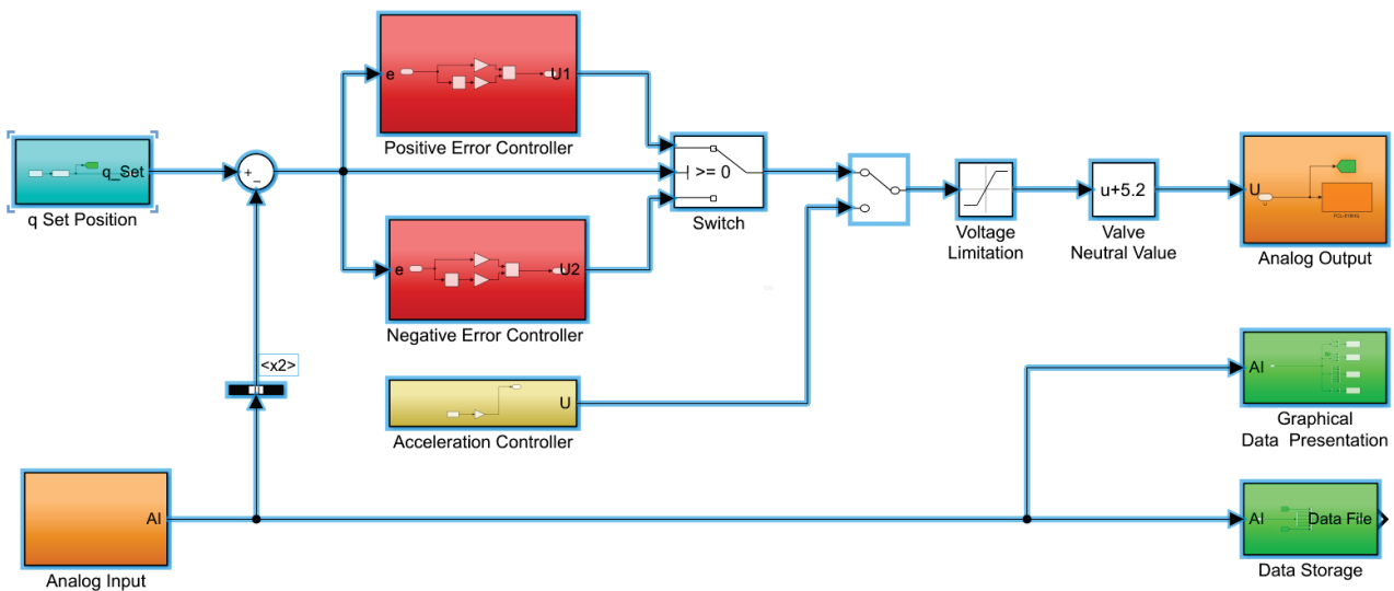
Fig. 6. Diagram of the control and data acquisition system implemented in MATLAB-Simulink Real-Time software
