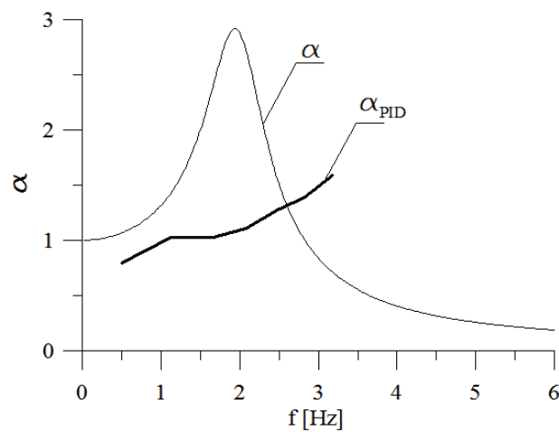
Fig. 8. Frequency response of passive and active systems
