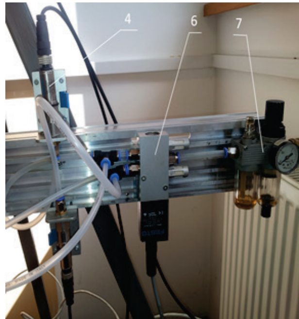
Fig. 5. View of the pneumatic control unit, pneumatic cylinder: 4 – pressure transducer, 6 – proportional directional control valve, 7 – air conditioner
