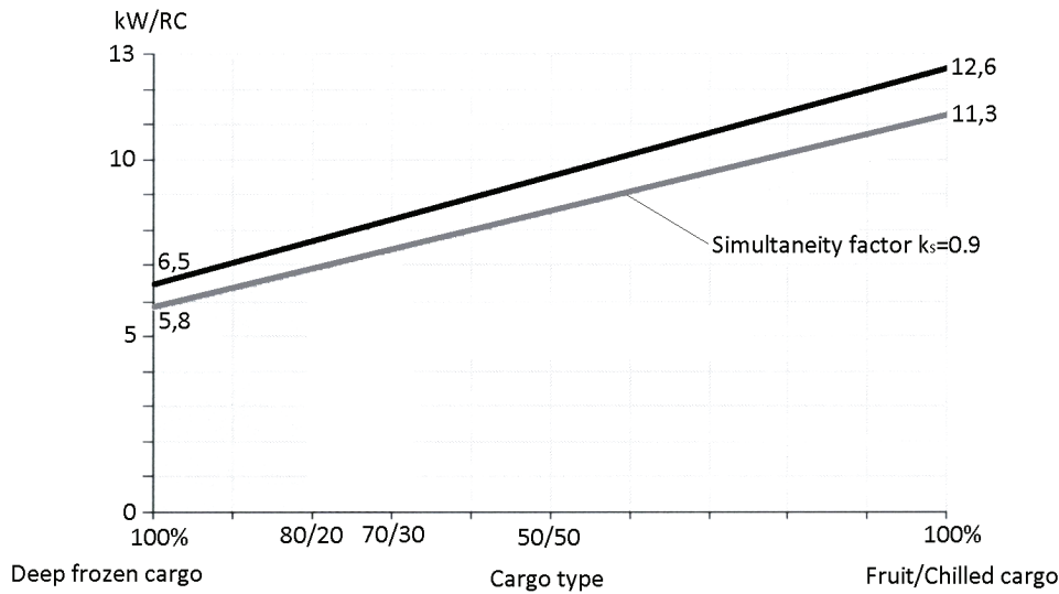
Fig.1. Electric power demand for reefer container 0
