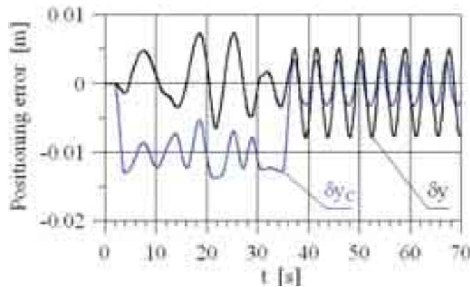
Fig 7. Positioning error
