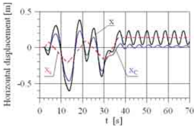
Fig. 6. Horizontal displacement
