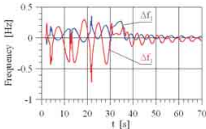
Fig. 9. Frequency correction
