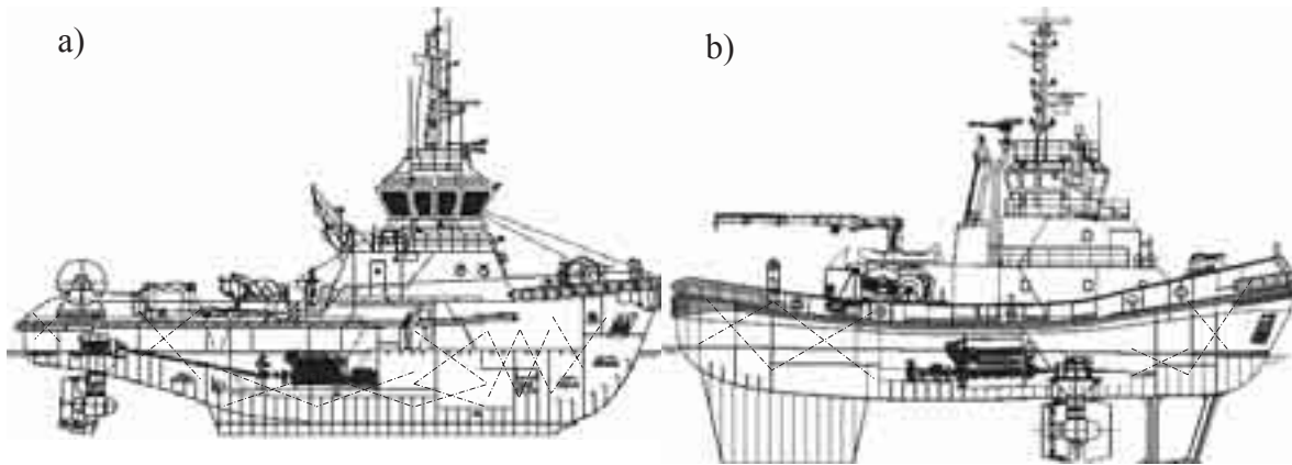
Fig. 1. Tug boats driven by azimuth thrusters. a) "pushing" type propulsion, b) "tractor" type propulsion
