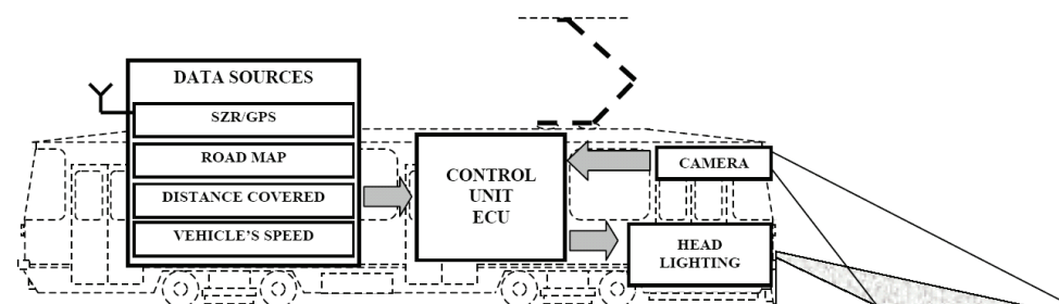
Fig. 1. Proposal for AFS system components for tram
